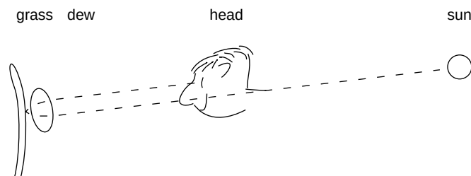
Figure 165 The path of light for dew on grass responsible for the aureole
