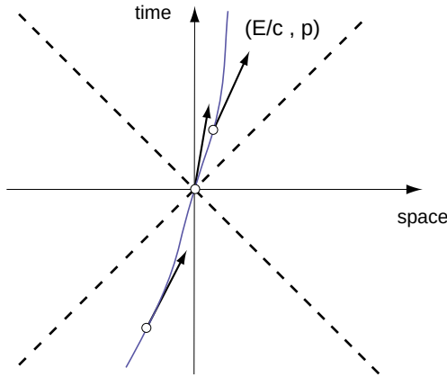
Figure 103 Energy-momentum is tangent to the world line
