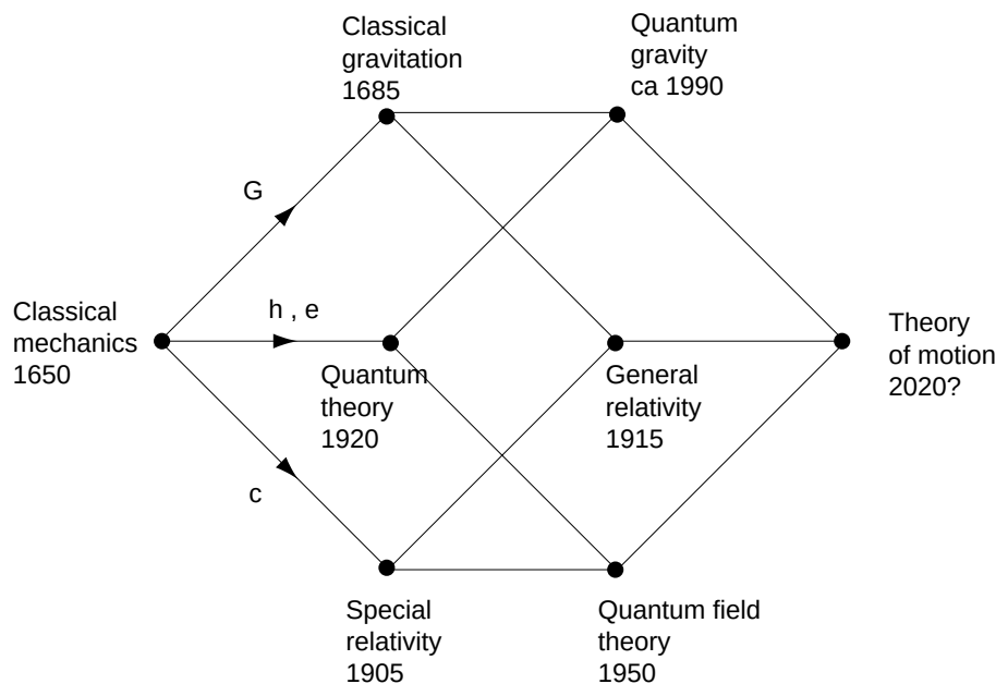
Figure 224 How the description of motion proceeded in the history of physics
