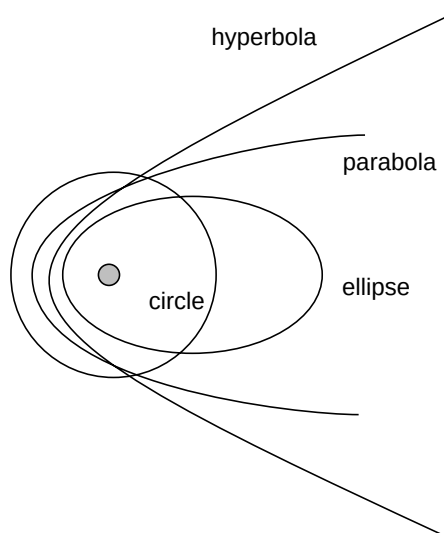
Figure 42 The possible orbits due to universal gravity
