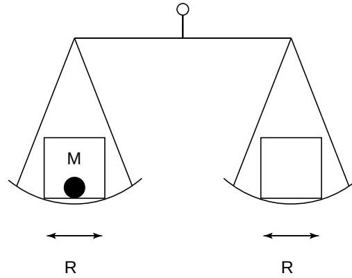
Figure 234 A Gedankenexperiment showing that at Planck scales, matter and vacuum cannot be distinguished
