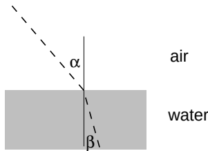
Figure 63 Refraction of light is due to travel time optimization
