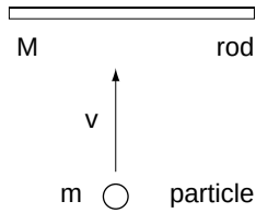
Figure 116 The reality of gravitomagnetism
