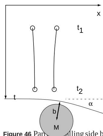
Figure 46 Partic falling side by side approach over time Figure 47 Masses bend light
