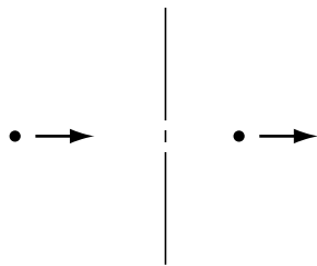
Figure 184 A particle and a screen with two nearby slits
