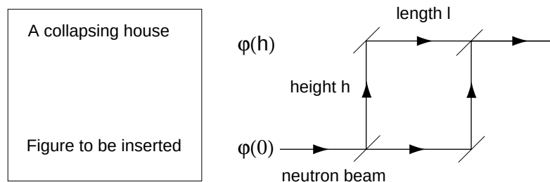
Figure 218 The weakness of gravitation
