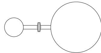
Figure 73 Which balloon wins?
