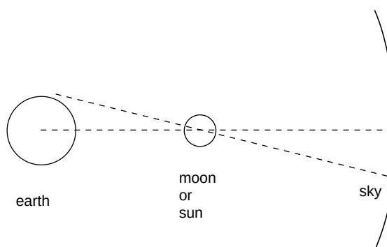
Figure 24 The parallax - obviously not drawn to scale
