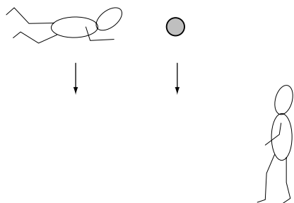
Figure 54 Can motion be described in a manner common to all observers?
