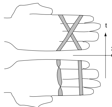
Figure 207 Equivalence of exchange and rotation in space-time
