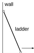
Figure 33 How does the ladder fall?
