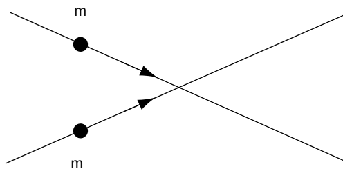
Figure 199 Identical objects with crossing paths – example, we saw that in a gas it is impossible to follow particles moving around and to say which particle is which.
