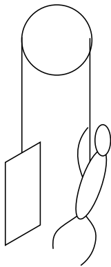
Figure 37 How does the ape move?
