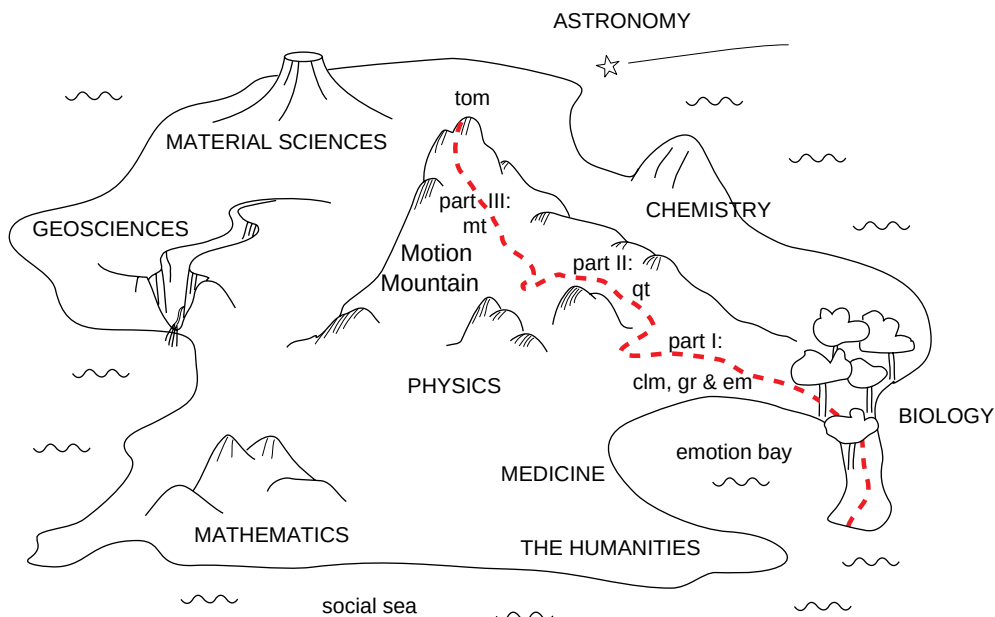
Figure 2 Experience Island, with Motion Mountain and the trail to be followed (clm: classical mechanics, gr: general relativity, em: electromagnetism, qt: quantum theory, mt: M-theory, tom: the theory of motion)
