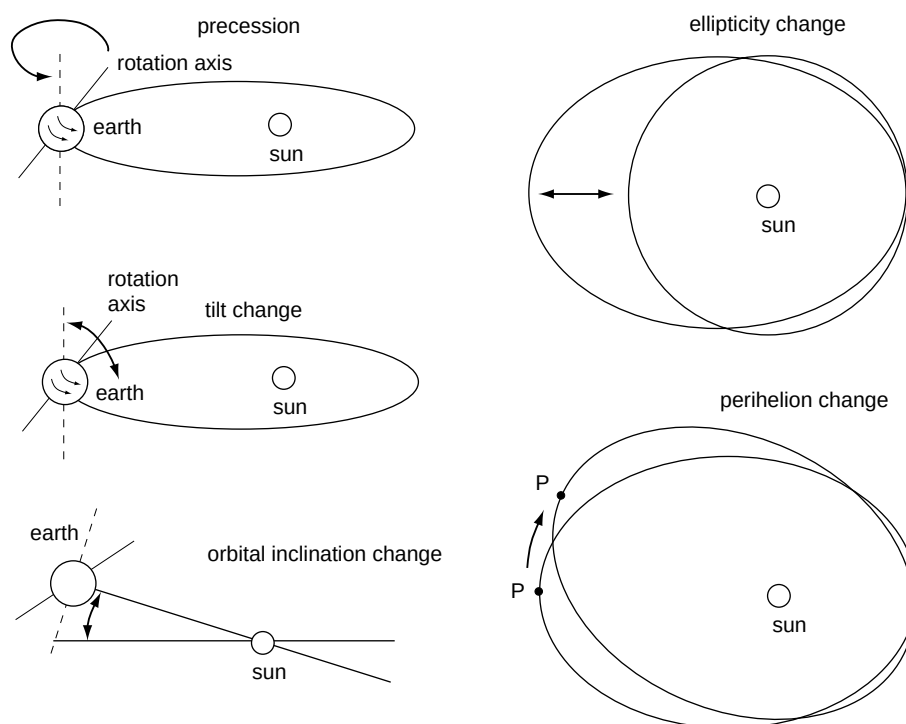
Figure 30 Changes in the earth's motion around the sun
