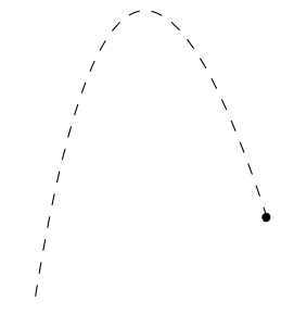
Figure 5 A typical path followed by a stone thrown through the air
