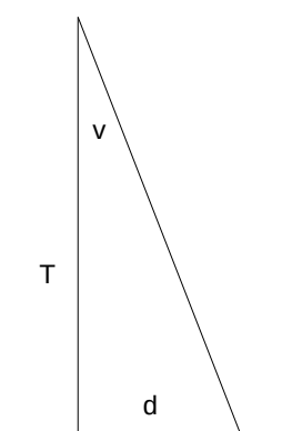
Figure 232 Trees and galaxies
