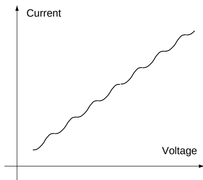
Figure 196 Steps in the flow of electrons Many electrons can move freely in metals; that is the reason that metal conduct electric current so well.
