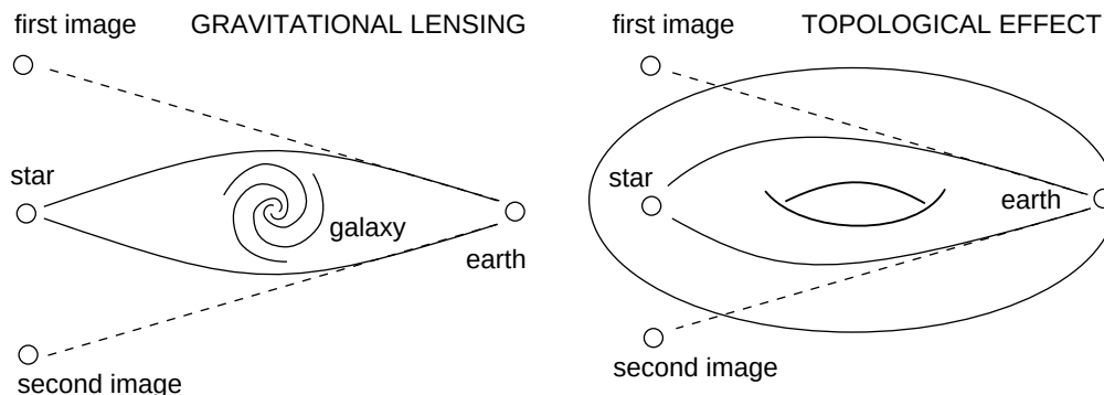
Figure 132 How one star can lead to several images
