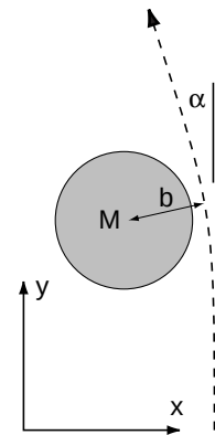
Figure 121 Calculating the bending of light by a mass
