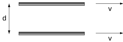
Figure 147 The relativistic aspect of magnetism
