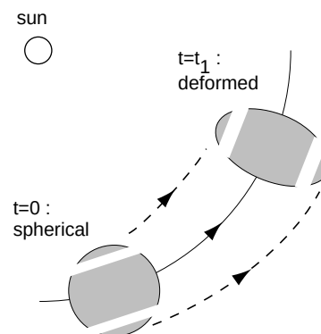
Figure 44 Tidal deformations due to gravity
